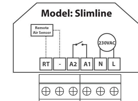
Wiring Detail
